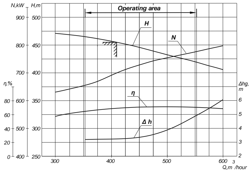
Performance and curves of NSSh 410-455 pump at the rotational speed n=24.59 \text{ s}^{-1} (1475 rpm) with water of density \rho=1000 \text{ kg/m}^3
