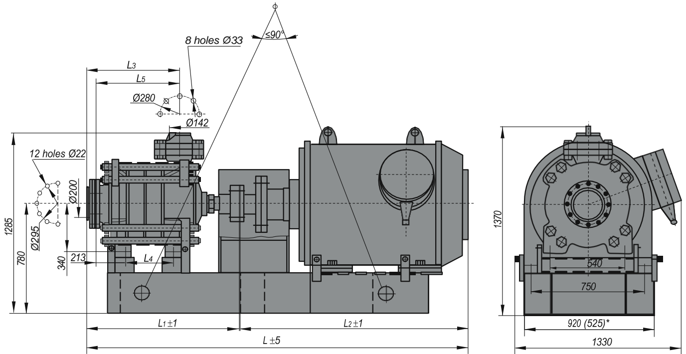
Overall dimensions and weight
