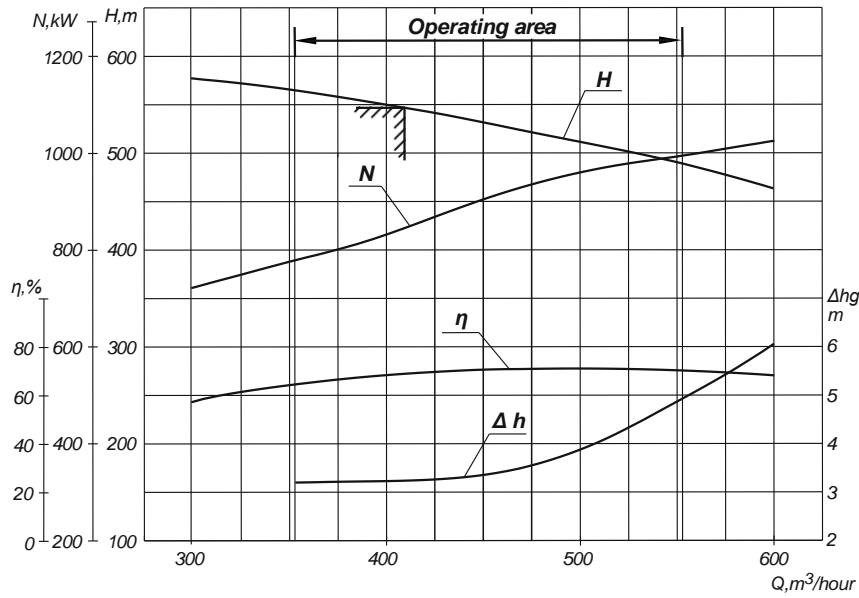
Performance and curves of NSSh 410-546 pump at the rotational speed n=24.59 \text{ s}^{-1} (1475 rpm) with water of density \rho=1000 \text{ kg/m}^3
