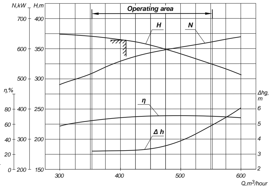
Performance and curves of NSSh 410-364 pump at the rotational speed n=24.59 \text{ s}^{-1} (1475 rpm) with water of density \rho=1000 \text{ kg/m}^3
