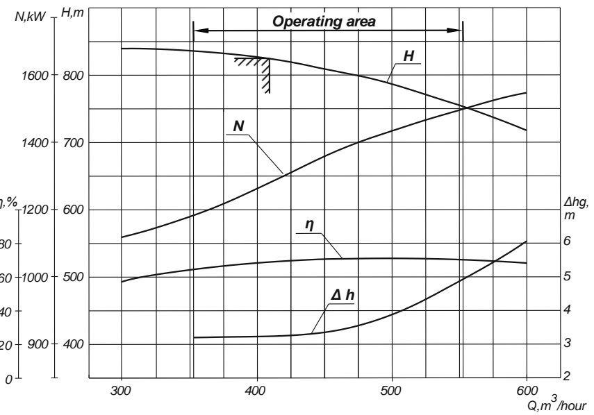
Performance and curves of NSSh 410-819 pump at the rotational speed n=24.59 \text{ s}^{-1} (1475 rpm) with water of density \rho=1000 \text{ kg/m}^3
