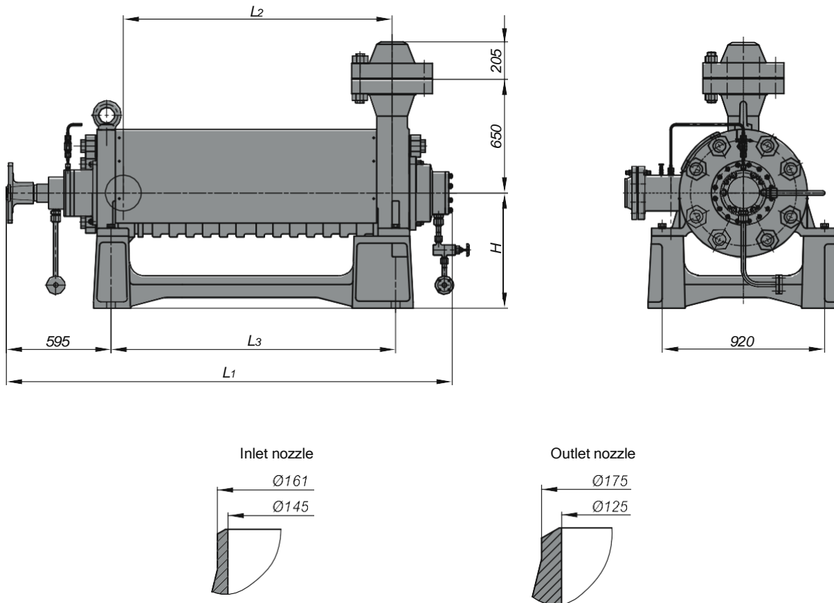
Dimensional drawing of CNS 120-...-3M, CNS 180-...-3T, CNS 240-...-3T-M pumps
