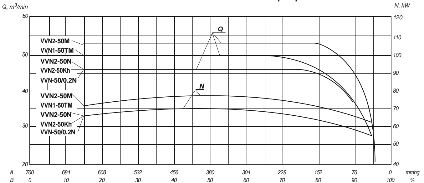
Performances and curves of pumps
