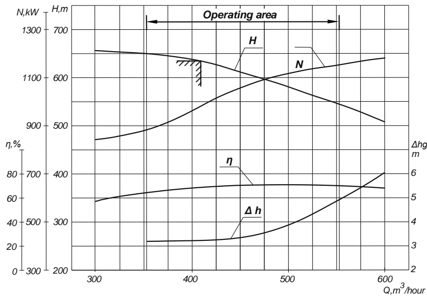
Performance and curves of NSSh 410-637 pump at the rotational speed n=24.59 \text{ s}^{-1} (1475 rpm) with water of density \rho=1000 \text{ kg/m}^3
