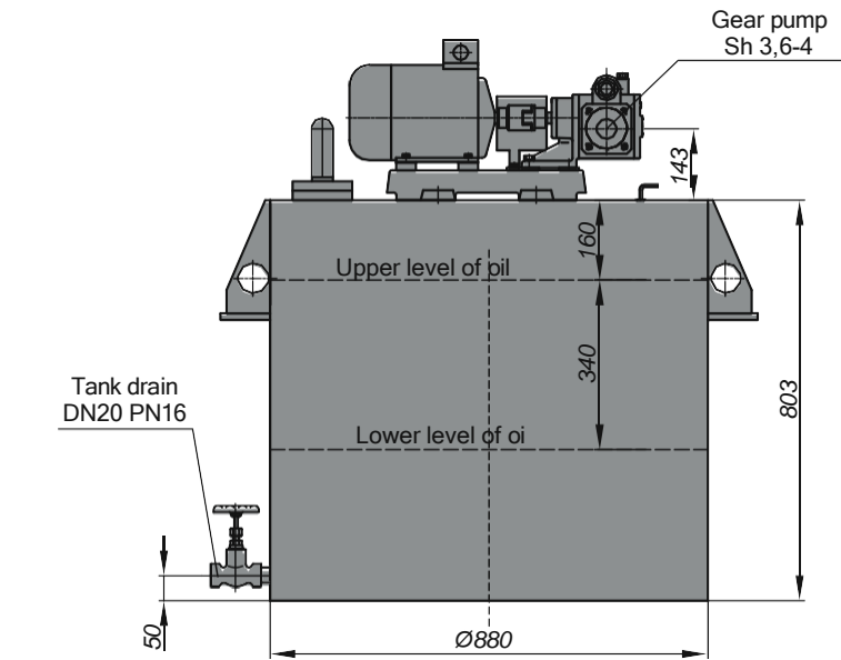
Oil tank BM-0,32
