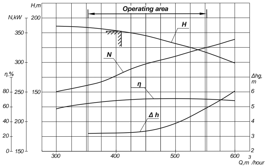
Performance and curves of NSSh 410-182 pump at the rotational speed n=24.59 \text{ s}^{-1} (1475 rpm) with water of density \rho=1000 \text{ kg/m}^3
