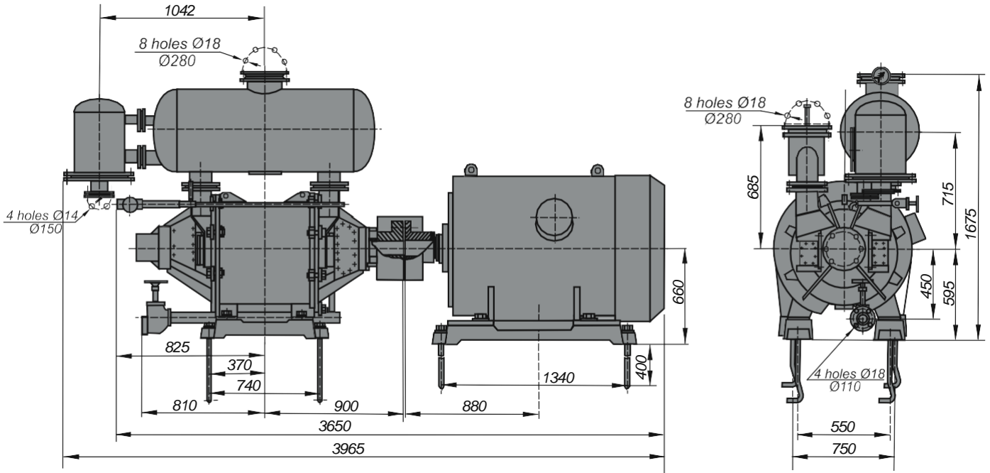
Dimensional drawing of VK-60/2.5N compressor
