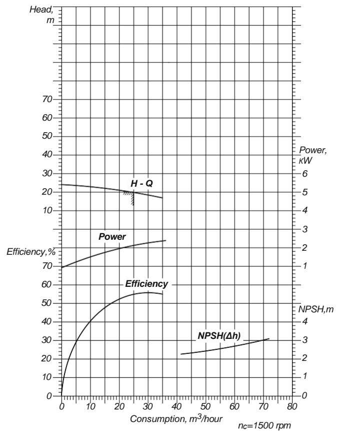
Performances and curves of electric pumping unit KhPE 80-50-250-D-55
