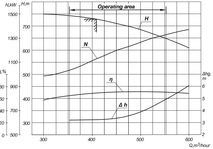
Performance and curves of NSSh 410-728 pump at the rotational speed n=24.59 \text{ s}^{-1} (1475 rpm) with water of density \rho=1000 \text{ kg/m}^3
