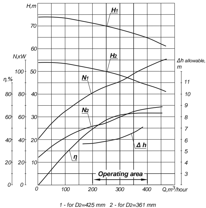
Performances and curves of CPN 225-70 pumping units at the rotational speed n=1480 rpm with water of density \rho = 998 kg/m 3
