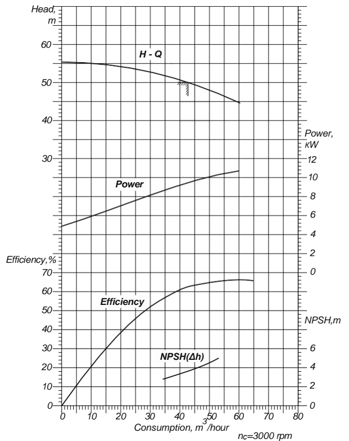
Performances and curves of electric pumping unit KhPV 80-50-200-D
