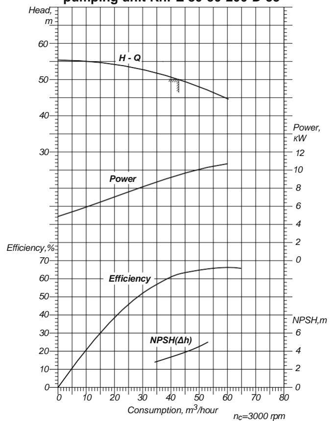
Performances and curves of electric pumping unit KhPE 80-50-200-D-55
