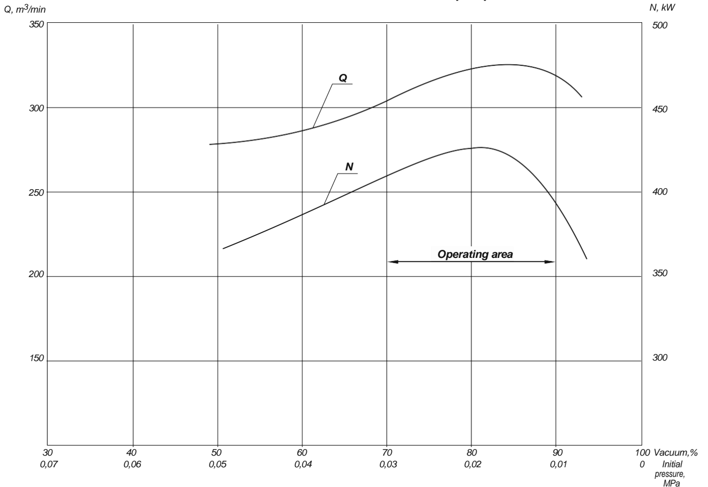
Performances and curves of VVN2-300 pump
