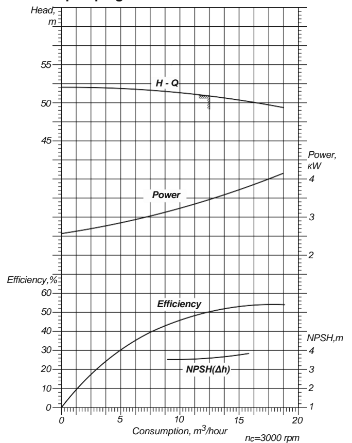
Performances and curves of electric pumping unit KhPE 50-32-200-D-55
