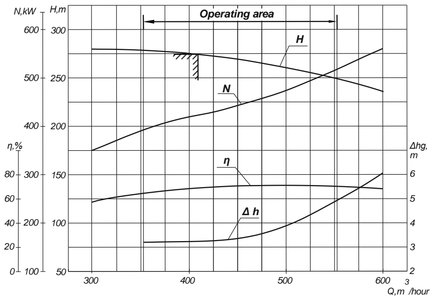
Performance and curves of NSSh 410-273 pump at the rotational speed n=24.59 \text{ s}^{-1} (1475 rpm) with water of density \rho=1000 \text{ kg/m}^3
